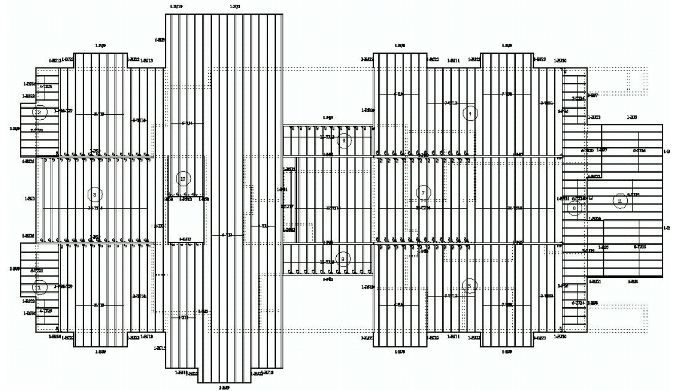
2D Board Layout with Key Labels
