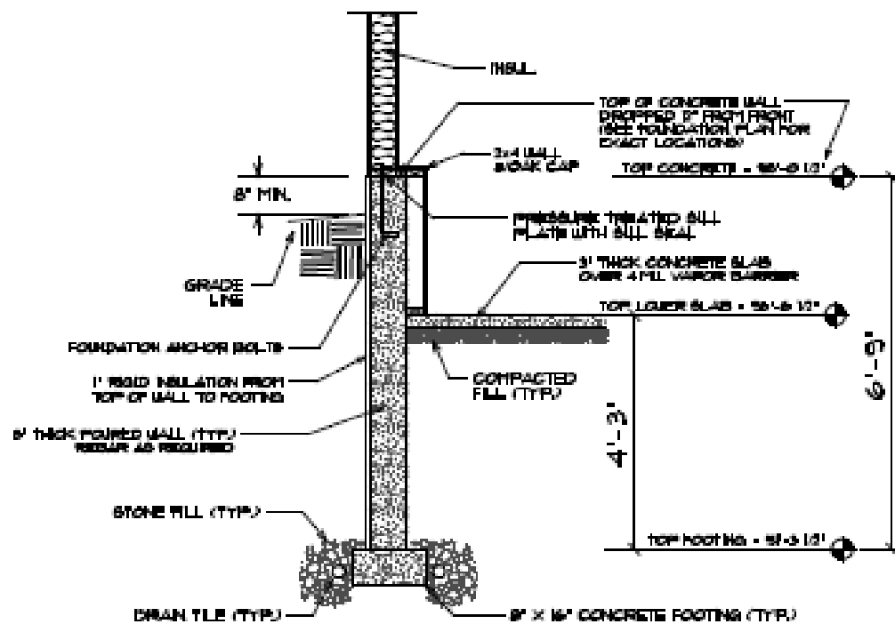
C FOUNDATION DETAIL F2 SCALE: 1/2" = 1'-0"
