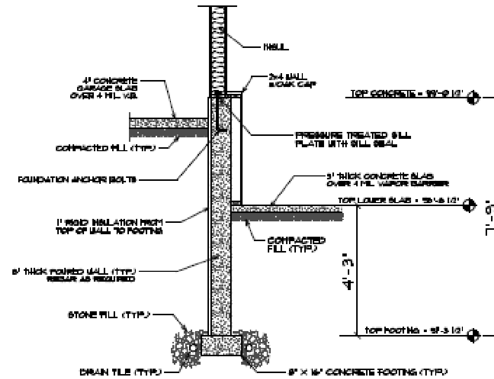
B FOUNDATION DETAIL F2 SCALE: 1/2" = 1'-0"
