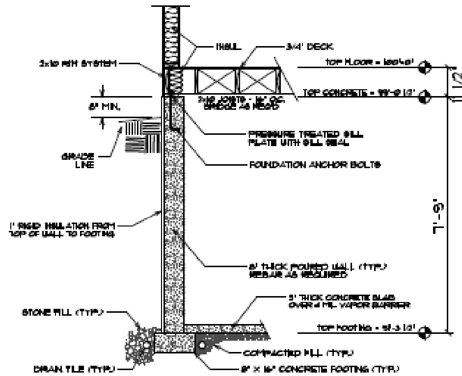
A FOUNDATION DETAIL F2 SCALE: 1/2" = 1'-0"
