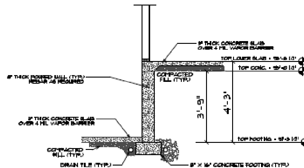
D FOUNDATION DETAIL F2 SCALE: 1/2" = 1'-0"
